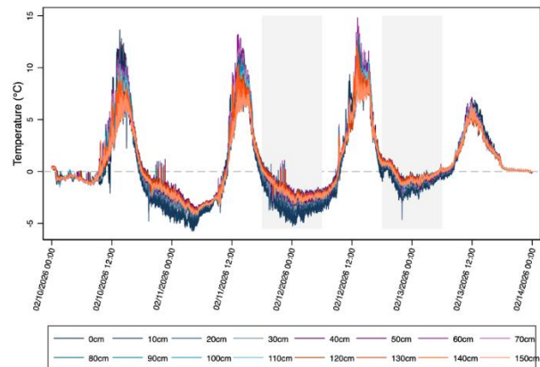
Figure 3: Thermocouple array data, Feb 10-13, 2026.
