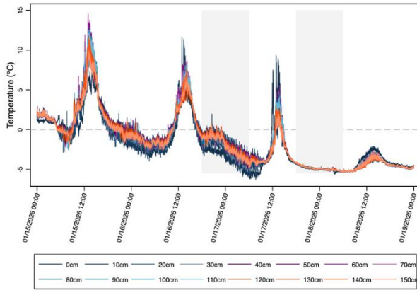
Figure 1: Thermocouple array data, Jan 15-18, 2026.
