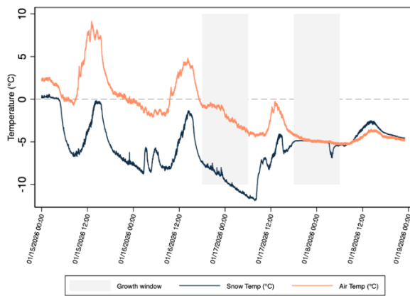
Figure 2: Air temperature and snow surface temperature, Jan 15-18, 2026.
