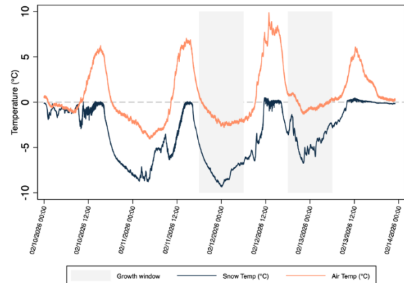
Figure 4: Air temperature and snow surface temperature, Feb 10-13, 2026.
